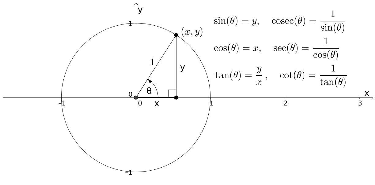
Figure 2: Definition of Trigonometric Functions.
